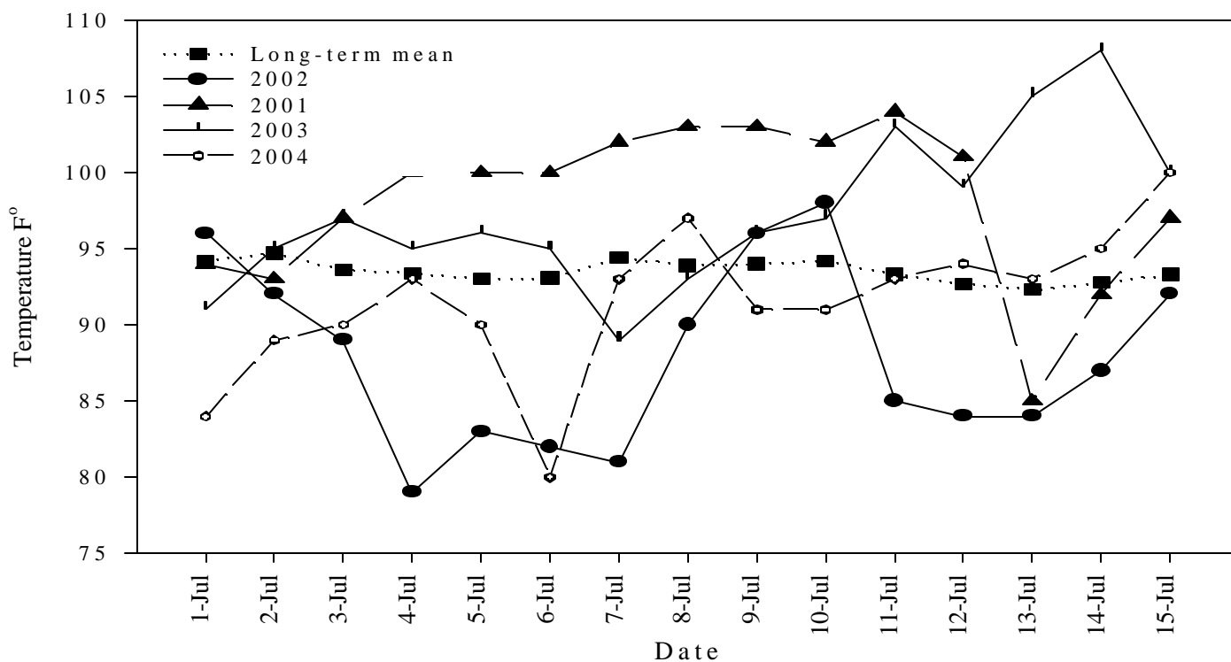
Figure 1. Daily OPREC high temperatures for July 1 through July 15, 2001 through 2004, and long-term mean.
